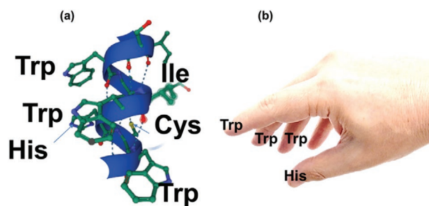
Figure 3. Structure of the selective binding pocket of WIWHCW. a) Helix structure of the peptide WIWHCW. b) Schematic presentation of the selective binding geometry as a gripping hand with Trp (W) and His (H) side chains as fingers.
