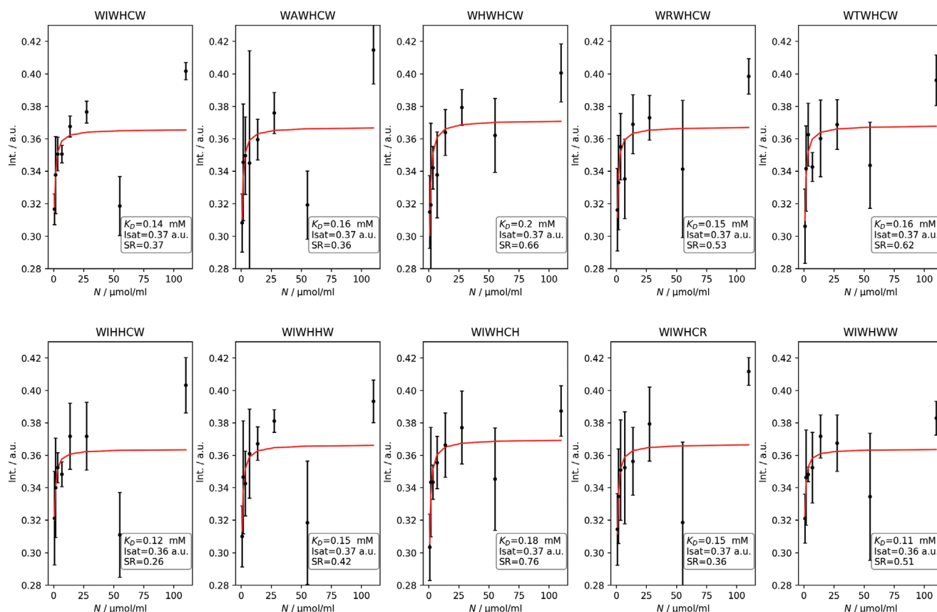
Figure 4. Fluorescence intensity (Int.) of the peptide spots for ten different peptides versus the different Nafion ionomer concentrations in ethanol. The signals (black dots with standard deviations) were fitted with the saturation curve (red line) according to the formula (1). An equilibrium dissociation constant K_D of 140 \mu\text{M} ( \text{SR} = 0.37 ) was obtained for the peptide WIWHCW.
