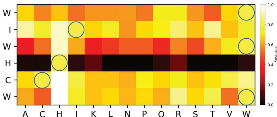
Figure 2. Substitutional analysis of the selective binder WIWHCW. Each pixel represents a peptide sequence where one of the amino acids from the WIWHCW is substituted against the other 14 shown on the horizontal axis. Blue circles indicate the location of the initial WIWHCW on the chip. The amino acid His is essential for selective binding. The intensity of the signal is given in arbitrary units.
