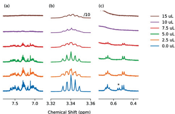
Figure 5. Titration of Cy5-WIWHCW with a 1/4 vol/vol Nafion/Methanol- d_4 solution. Panels (a), (b), and (c) show the aromatic region of the ^1H spectrum near 7 ppm, the residual solvent signal at 3.34 ppm, and methyl signals of isoleucine near 0.5 ppm, respectively. Adding the 1/4 vol/vol Nafion/Methanol- d_4 solution leads to significant broadening in the aromatic and methyl regions of the peptide spectrum. The broadening of the solvent signal in panel (b) is insignificant by comparison. Note that panels (a) and (c) span a chemical shift range of the order of 0.4 ppm, whereas panel (b) spans a ten times smaller range. Spectra are offset vertically for clarity.
