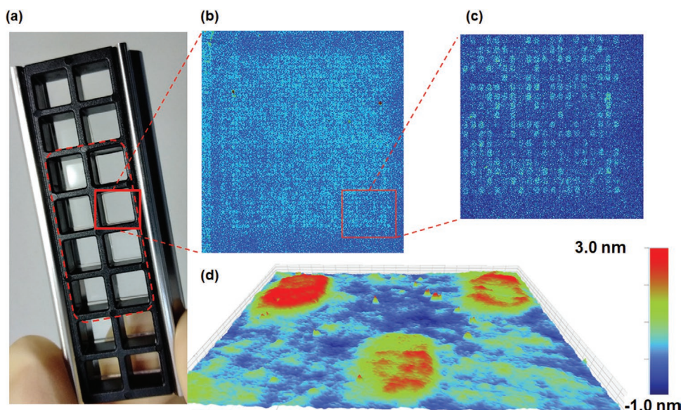
Figure 1. Alignment of the eight identical peptide libraries for substitution analysis and measurement of dissociation constants. a) Photo of a peptide chip in the incubation tray. The eight wells in the middle (dashed red line) were used to incubate the Nafion ionomer at eight concentrations to determine the dissociation constant. b and c) A fragment of fluorescence images of peptide libraries after incubation and its magnification. d) Profiles of the ionomer film accumulated on six peptide spots with different affinity to Nafion measured with a vertical scanning interferometer (three of the spots had no Nafion adhesion). The ionomer thickness on the peptide spot with the highest affinity (upper left corner) is <2 nm). The surface roughness of the peptide chip is \approx 1.5 nm.
